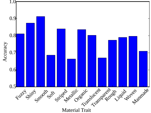
Figure 5. Visual material trait recognition accuracy. Material traits are recognized via binary classification on a balanced training and testing set, thus random chance accuracy is 50%. Most traits are recognized well. Difficult material traits, such as metallic and transparent, are challenging due to their object- and environment-dependent appearances. Average accuracy is 78.4%.
