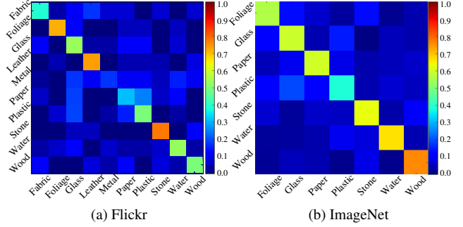
Figure 8. Confusion matrices showing true class vs. predicted class on the Flickr Material Database and ImageNet images. Average accuracy is 49.2% in (a) and 60.5% in (b). Though metal and glass both have an appearance that is environment-dependent, glass is more accurately classified. This is likely due to the tendency of glass to create characteristic local distortions.
