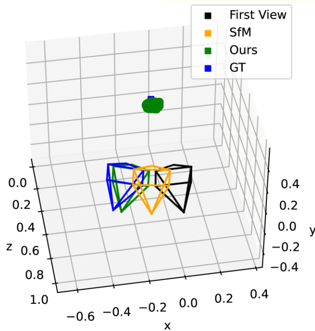
Recovered camera pose
